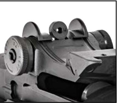
MATCH-GRADE NON-HOODED .0520 APERTURE, 1/2 MOA ADJ FOR WINDAGE & MOA FOR ELEVATION
