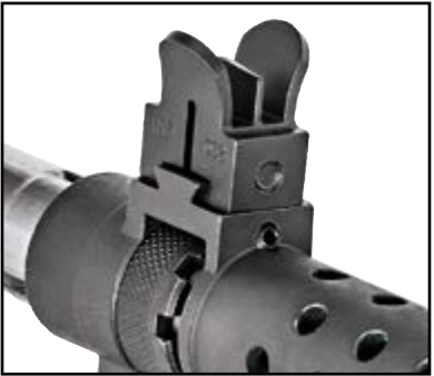
NATIONAL MATCH .062" BLADE FRONT SIGHT
